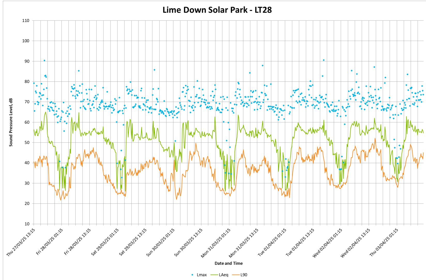
Plate 27: LT28 Measurement Time History (Cable Route Corridor)
