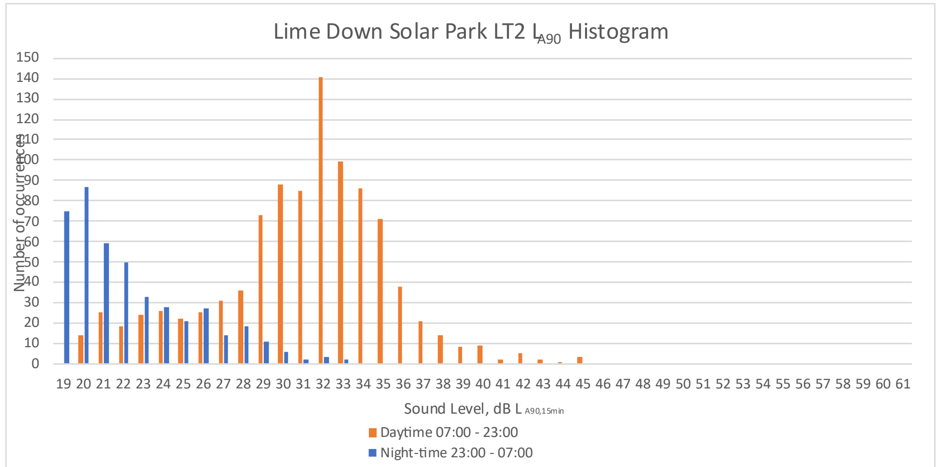
Plate 30: LT2 LA90 Histograms (Solar PV Sites)
