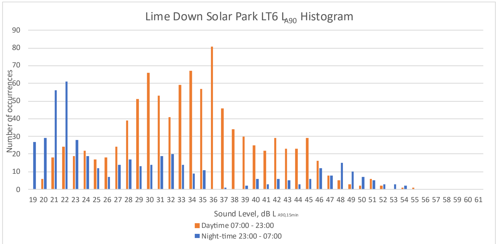
Plate 34: LT6 LA90 Histograms (Solar PV Sites)
