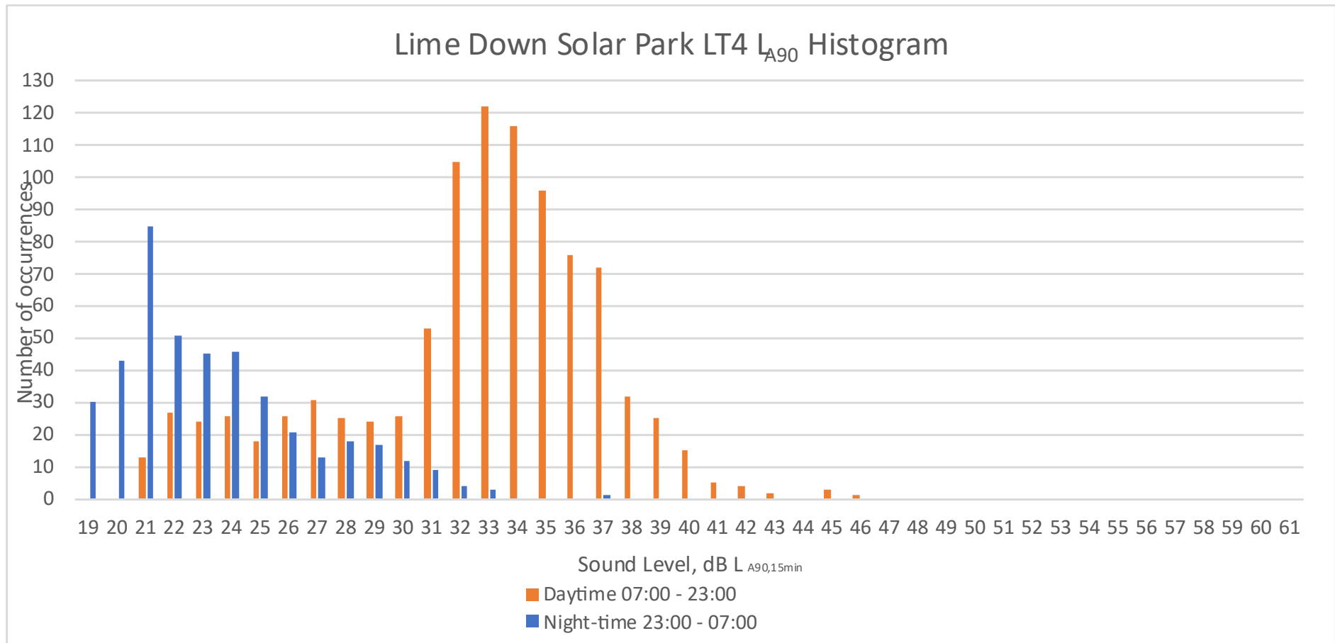
Plate 32: LT4 LA90 Histograms (Solar PV Sites)
