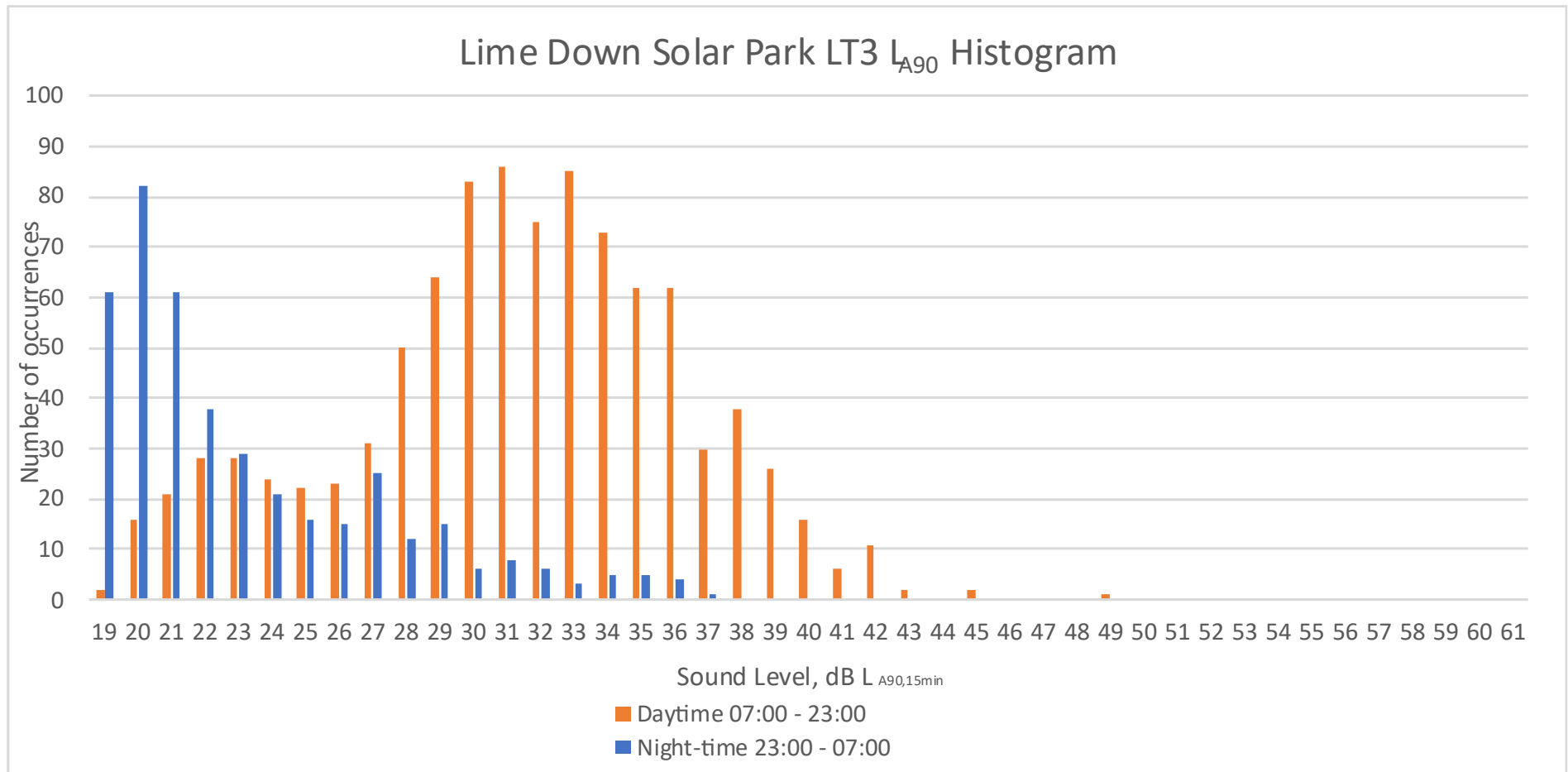
Plate 31: LT3 LA90 Histograms (Solar PV Sites)
