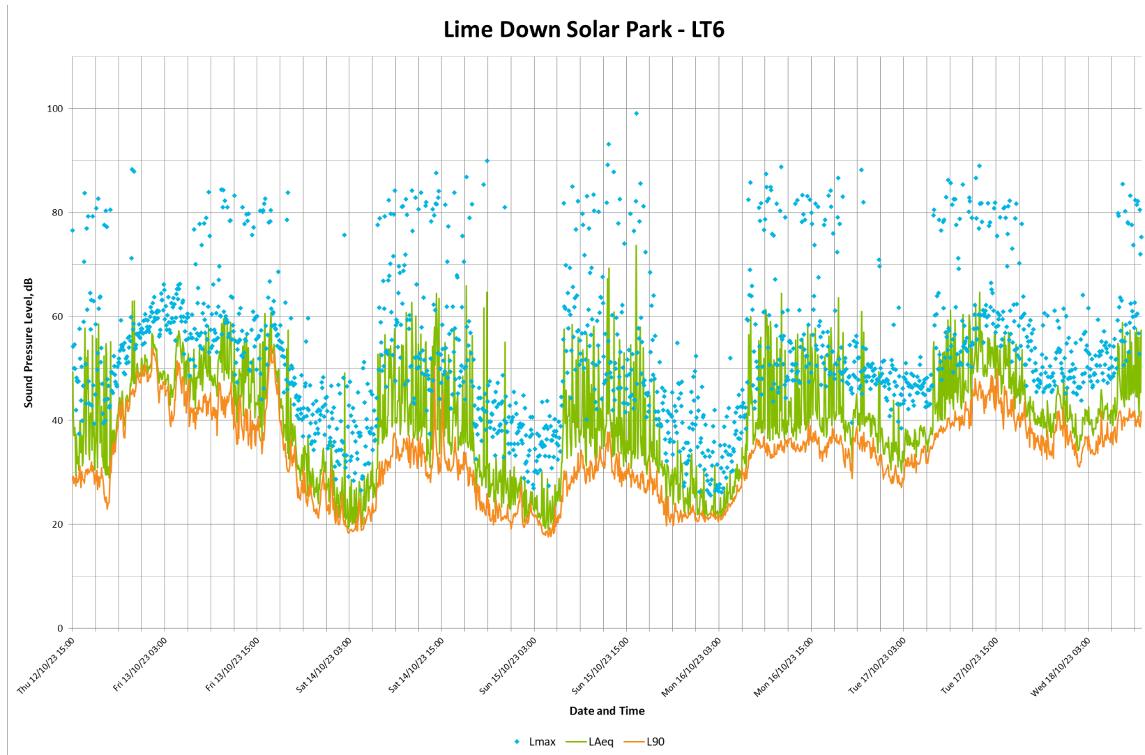
Plate 6: LT6 Measurement Time History (Solar PV Sites)
