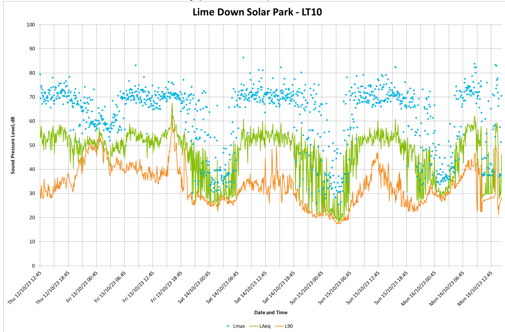
Plate 10: LT10 Measurement Time History (Solar PV Sites)
