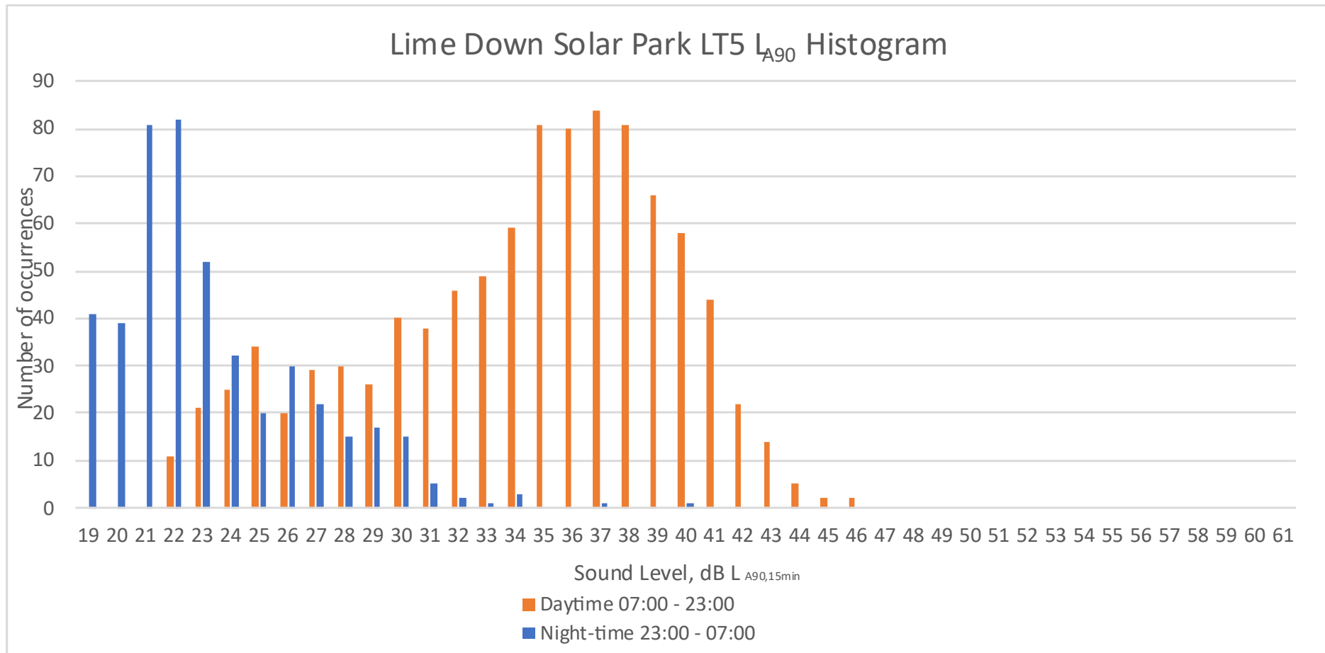
Plate 33: LT5 LA90 Histograms (Solar PV Sites)
