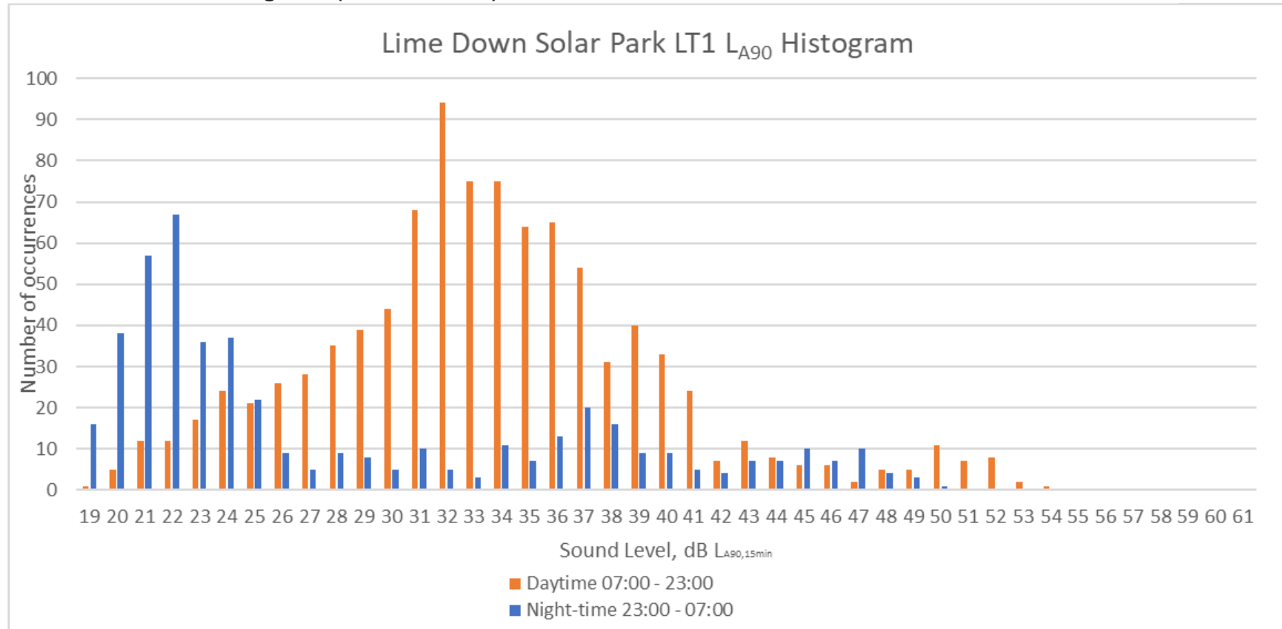
Plate 29: LT1 LA90 Histograms (Solar PV Sites)
