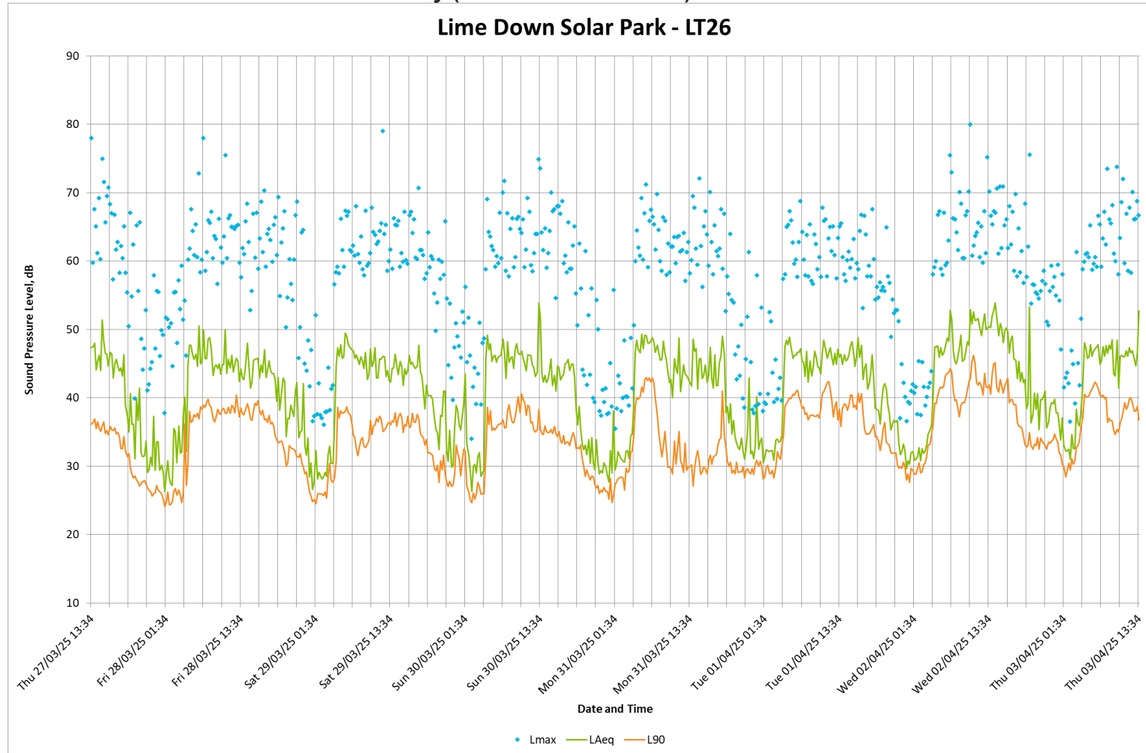
Plate 25: LT26 Measurement Time History (Cable Route Corridor)
