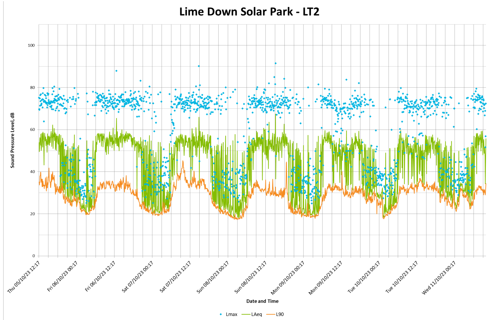
Plate 2: LT2 Measurement Time History (Solar PV Sites)
