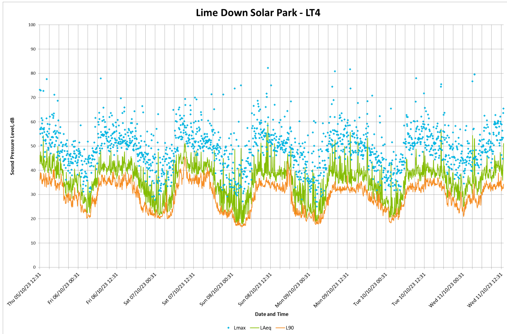
Plate 4: LT4 Measurement Time History (Solar PV Sites)
