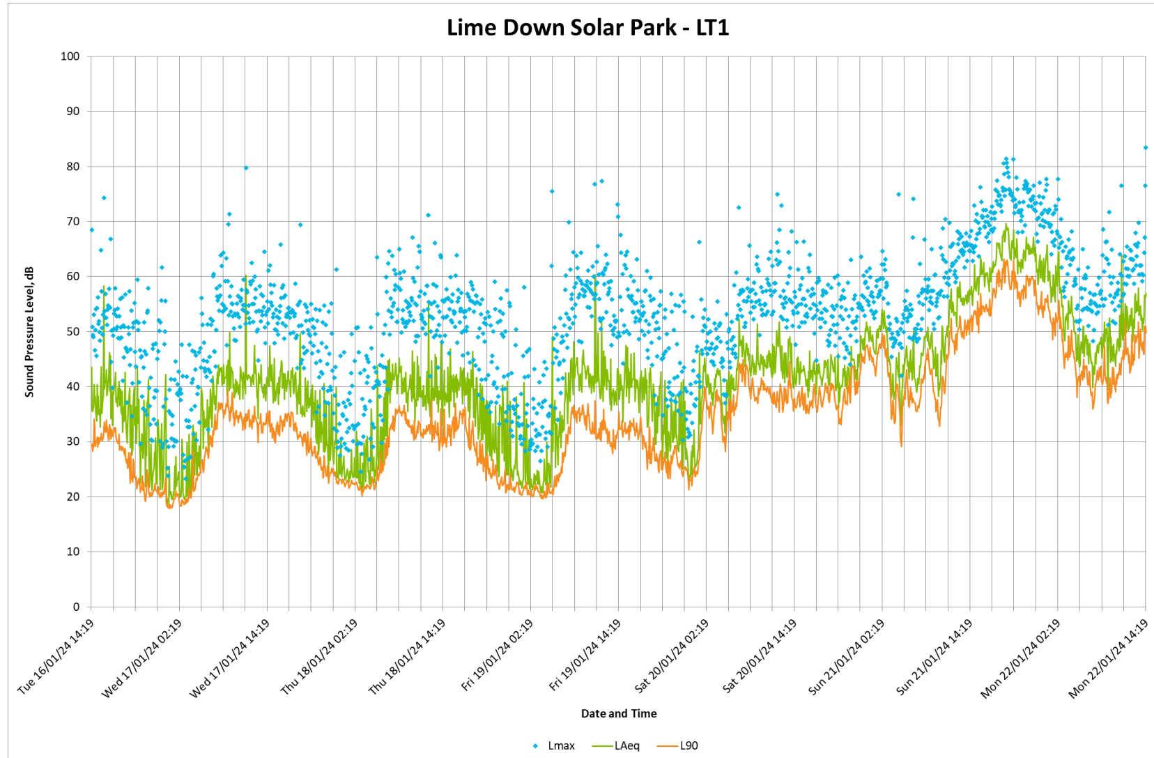
Plate 1: LT1 Measurement Time History (Solar PV Sites)
